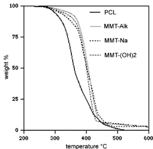
Fig. 3. Temperature dependence of weight loss under an air flow, for unfilled PCL and PCL-based nanocomposites prepared from the masterbatches M1–M3, and containing 3 wt% of inorganics (heating rate: 20 K/min).
