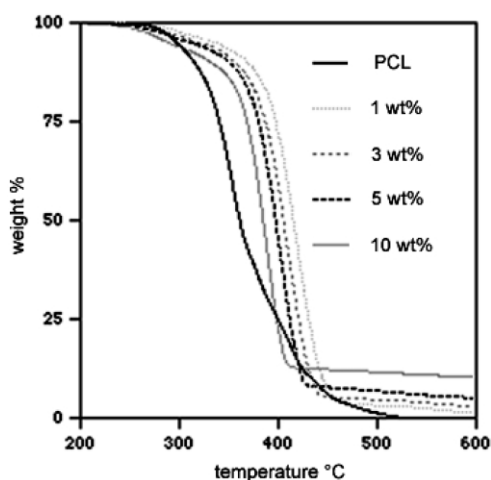
Fig. 4. Temperature dependence of weight loss under an air flow, for unfilled PCL and PCL-based nanocomposites prepared from the masterbatch (M1) and filled with 1, 3, 5 and 10 wt% of inorganics (heating rate: 20 K/min).
